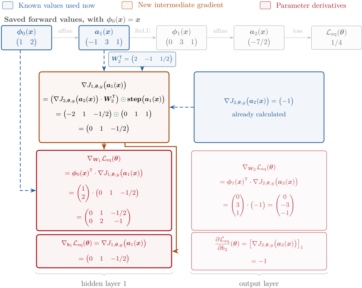
Figure 11: Step 2: calculate the hidden layer's derivatives. The blue row from the preceding step is multiplied by \mathbf{W}_2^\top . The componentwise product with \text{step}(\mathbf{a}_1(\mathbf{x})) = \begin{pmatrix} 0 & 1 & 1 \end{pmatrix} gives the orange row. This row gives the bias gradient and, together with \phi_0(\mathbf{x}) , the weight gradient. Every parameter derivative is now shown in red.
