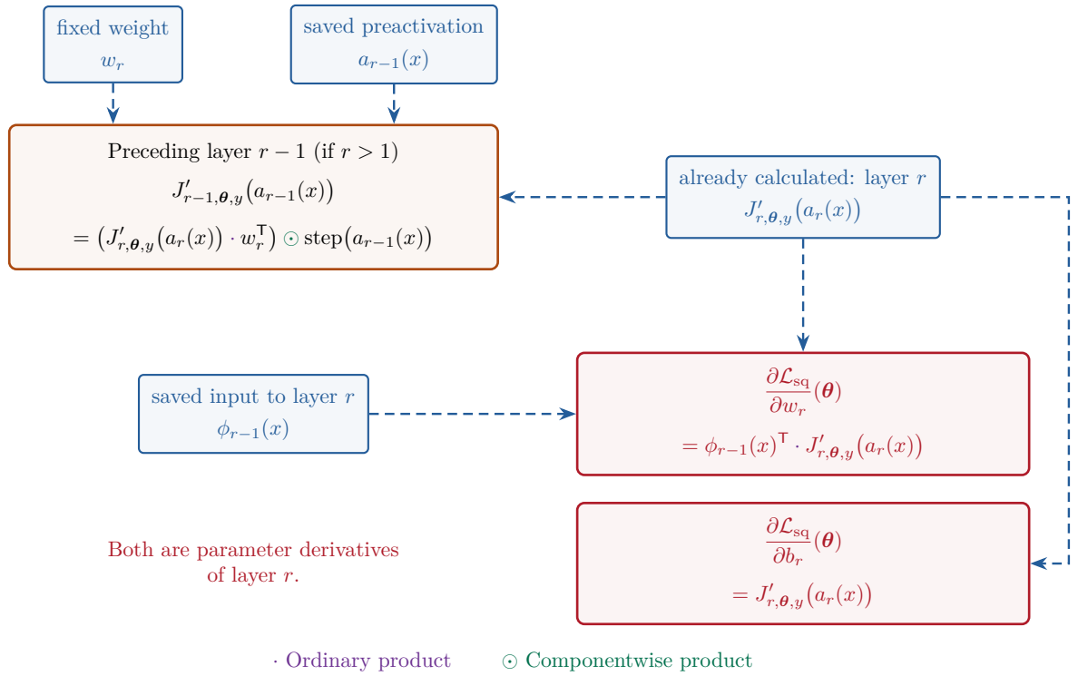
Figure 7: The scalar backward step from Figure 3, with products and transposes displayed to match the vector formulas. Purple \cdot marks ordinary matrix multiplication, and green \odot marks componentwise multiplication. Scalars are identified with 1 \times 1 matrices: both products multiply single entries, and transposition leaves them unchanged. Hidden preactivations are assumed nonzero.
