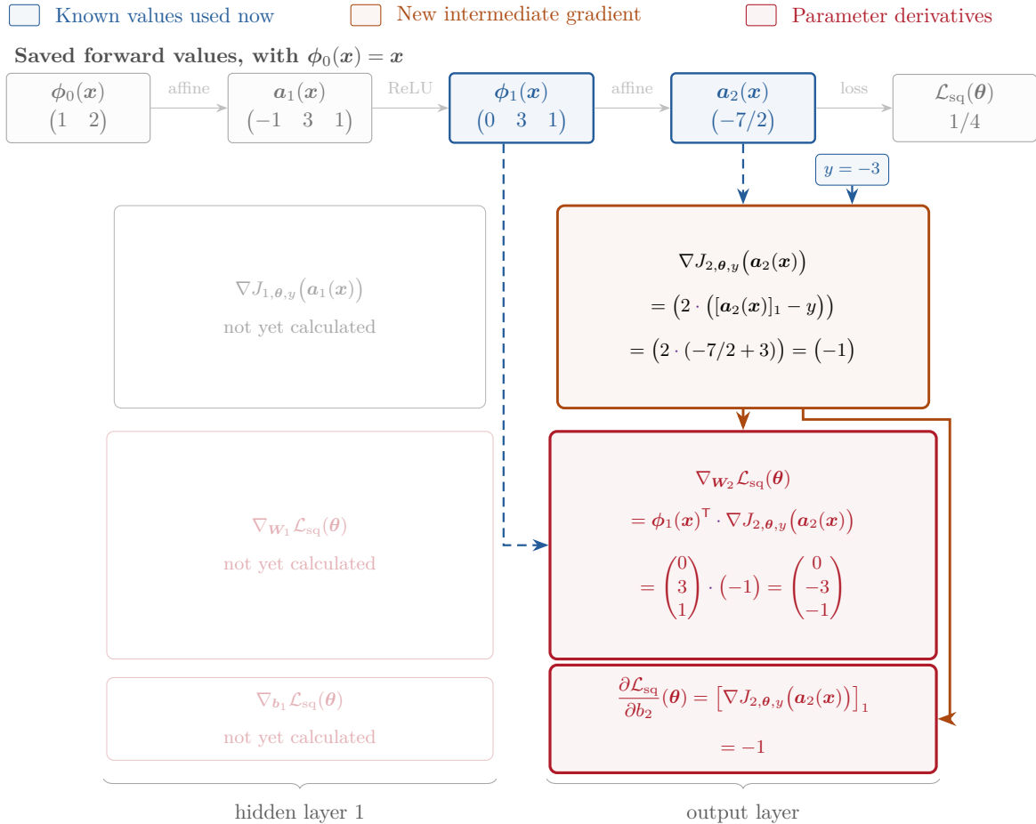
Figure 10: Step 1: calculate the output layer's derivatives. The saved output and target give the orange row. That row and the saved feature row \phi_1(\mathbf{x}) both enter the weight-gradient calculation. The single entry of the orange row also gives the derivative with respect to the scalar bias b_2 .
