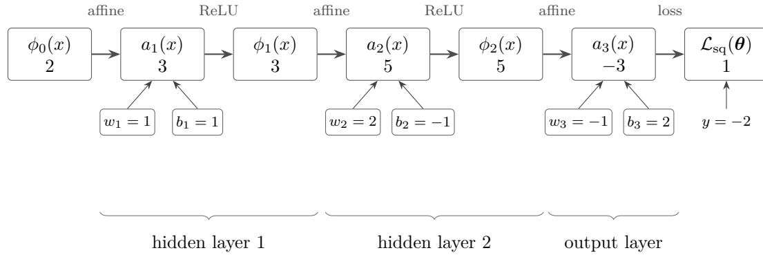
Figure 1: The scalar forward pass for the observation and parameters in (3). The lower braces identify the two hidden layers and the output layer. The loss is calculated after the network has produced its prediction.
