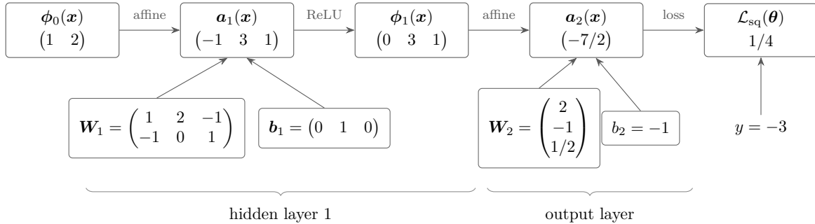
Figure 9: The forward pass for the network in (21). The input has two coordinates, the hidden layer produces three features, and the output row has one coordinate. The weights and biases enter their affine calculations, while the target enters the squared loss. These forward values are kept for the backward pass.
