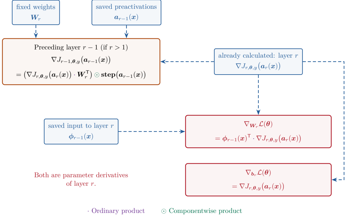
Figure 8: The backward pass proceeds from right to left. The blue gradient at layer r is reused to calculate the two red parameter gradients below it and the orange gradient for layer r - 1 to its left. The orange result is reused at the next backward step. As in Figure 7, purple \cdot marks ordinary matrix multiplication and green \odot marks componentwise multiplication. Here step applies the scalar step function to each coordinate. Every hidden preactivation coordinate is assumed nonzero.
