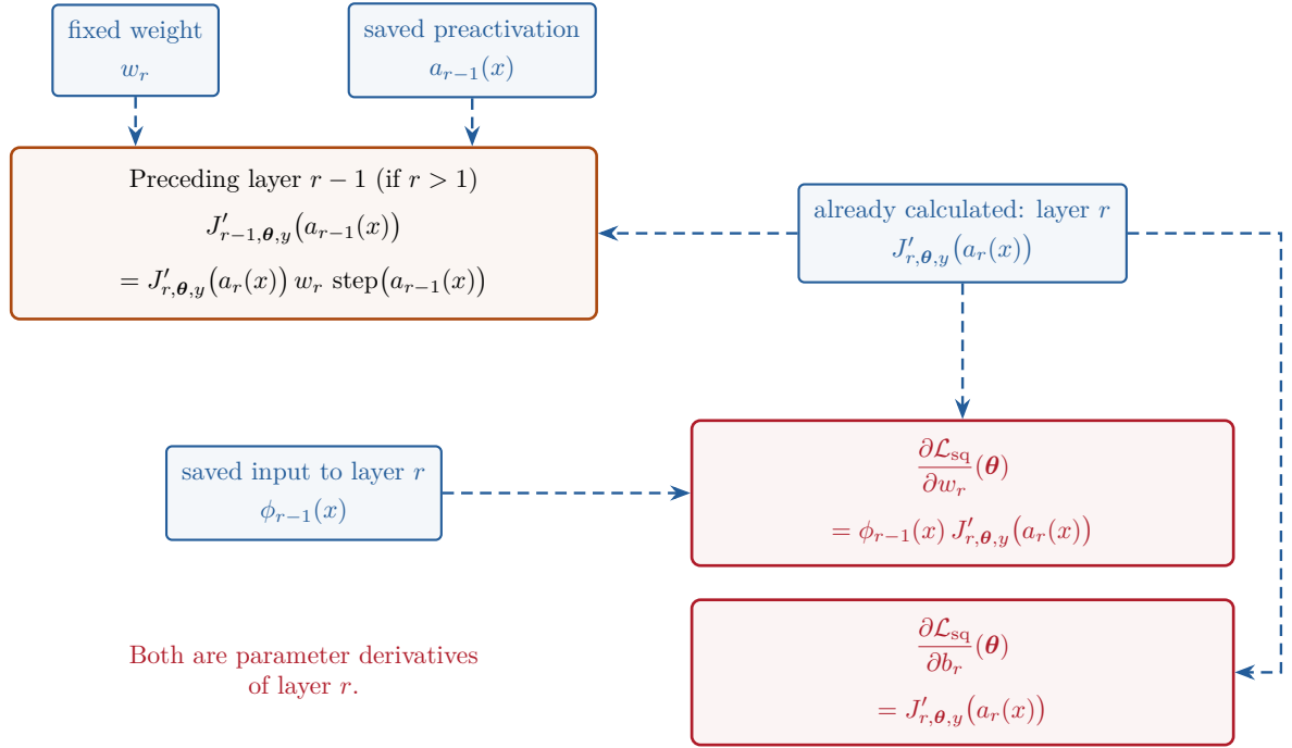
Figure 3: Reusing one intermediate derivative in the scalar network. For r = 1, 2, 3 , the blue value on the right gives the two red parameter derivatives below it. If r > 1 , it also gives the orange derivative for the preceding layer, using the fixed weight and saved preactivation above. That orange value becomes the blue input at the next step. Both hidden preactivations are assumed nonzero.
