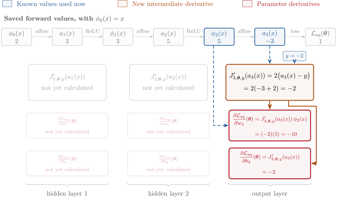
Figure 4: Step 1: the output layer. The prediction a_3(x) and target y give J'_{3,\theta,y}(a_3(x)) . This is the derivative with respect to b_3 . Multiplying it by the saved input \phi_2(x) gives the derivative with respect to w_3 .
