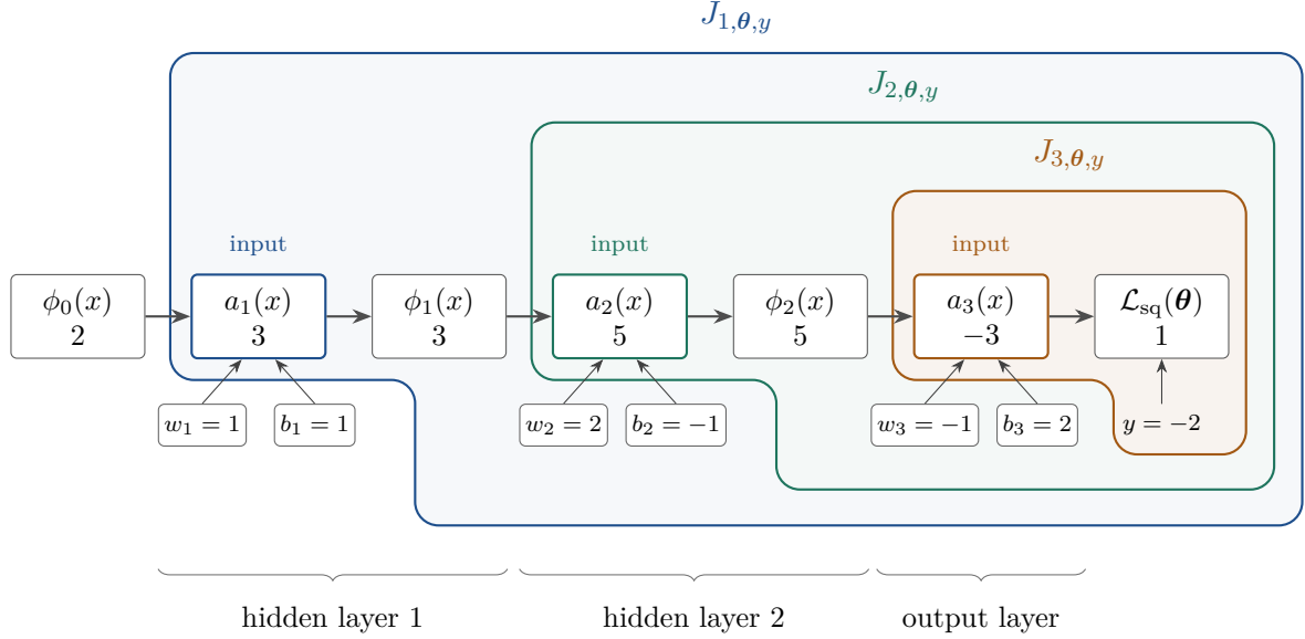
Figure 2: The forward pass at the parameters in (3). Each coloured region represents one remaining function, evaluated at the input marked in the same colour. Its calculation uses that input and the quantities inside the region. The earlier quantities affect the result only through the supplied input value.
