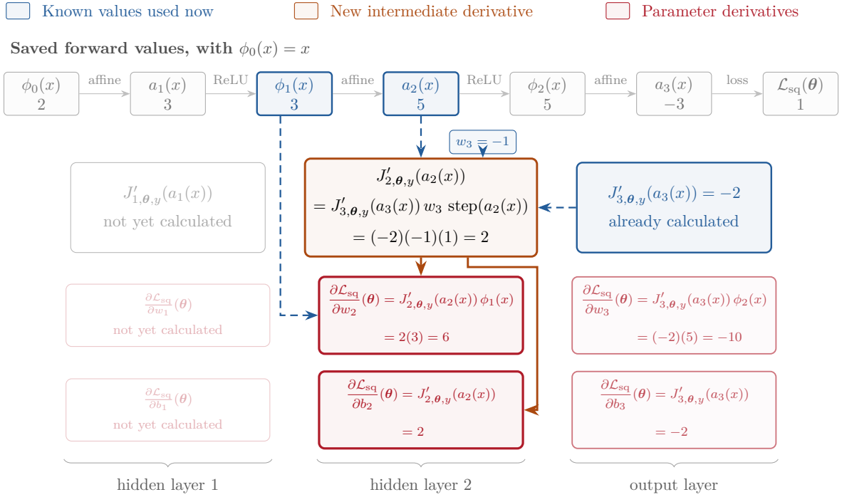
Figure 5: Step 2: the second hidden layer. We reuse J'_{3,\theta,y}(a_3(x)) , together with w_3 and a_2(x) , to calculate J'_{2,\theta,y}(a_2(x)) . This gives the bias derivative directly and, after multiplication by the saved input \phi_1(x) , the weight derivative.
