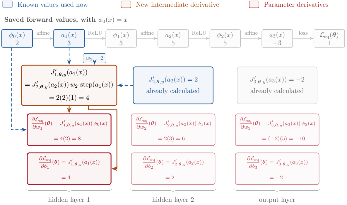
Figure 6: Step 3: the first hidden layer. We reuse J'_{2,\theta,y}(a_2(x)) , together with w_2 and a_1(x) , to calculate J'_{1,\theta,y}(a_1(x)) . The layer input is \phi_0(x) = x , so the same rule gives the final two parameter derivatives. All six required derivatives are now shown in red.
